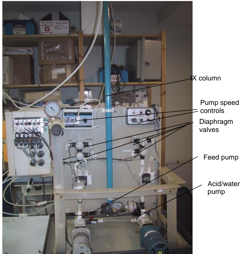
Figure 2: IX Pilot Plant
